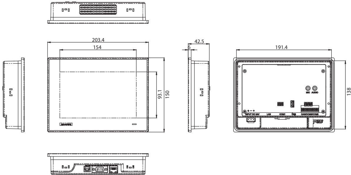
Panel Cut Out Dimensions: 192 x 138.5 mm (7.56" x 5.45")
